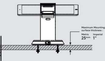
Mounting: Fixing from Below
